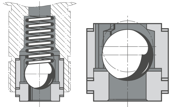
Ball valve
