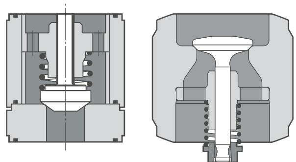
Cone valve
