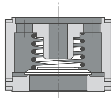
Disc valve
